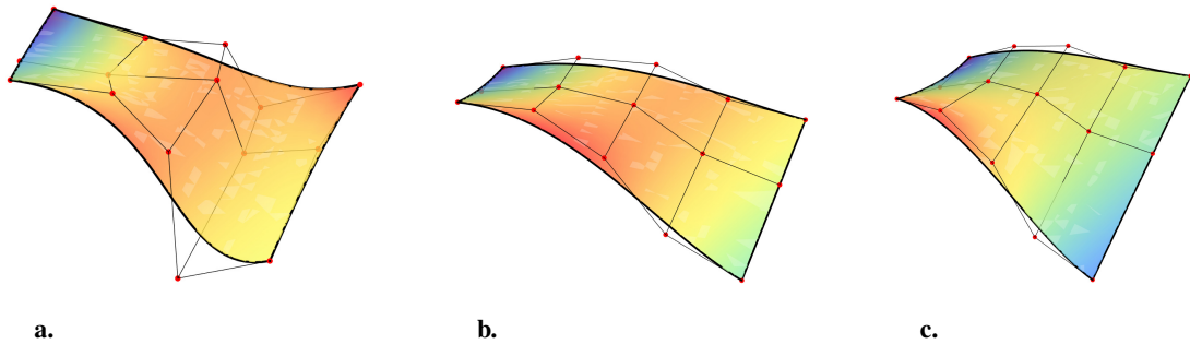
Figure 2: (illustrates examples 1 and 2) Three irreducible TPB surfaces of degree (4, 2) with control points shown in Table 1. a. Surface S_1 ; b. Surface S_2 ; c. Surface S_3 ;
