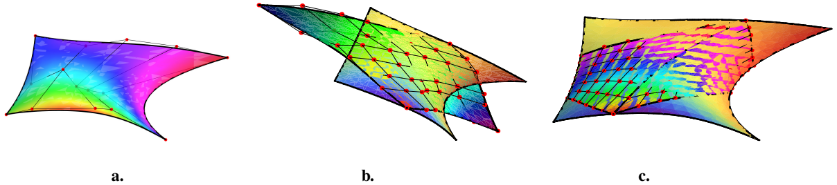
Figure 6: a. Irreducible TPB surfaces S_1 of degree (2, 4) and S_2 of degree (6, 6) from Example 5. The control points of S_1 and S_2 are shown in Table 3. a. S_1 ; b. S_1 and S_2 with its control polygon; c. The coincident part S is presented as two TPB surfaces.
