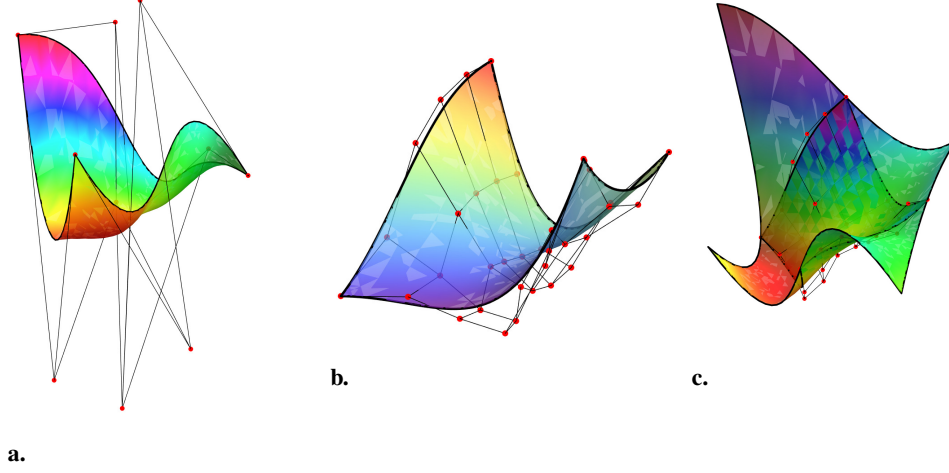
Figure 4: The irreducible TPB surfaces S_1 of degree (2, 3) and S_2 of degree (5, 5) from Example 3. The corresponding control points are shown in Table 2. a. Surface S_1 ; b. Surface S_2 ; c. The coincident part of S_1 and S_2 is S_2 .
