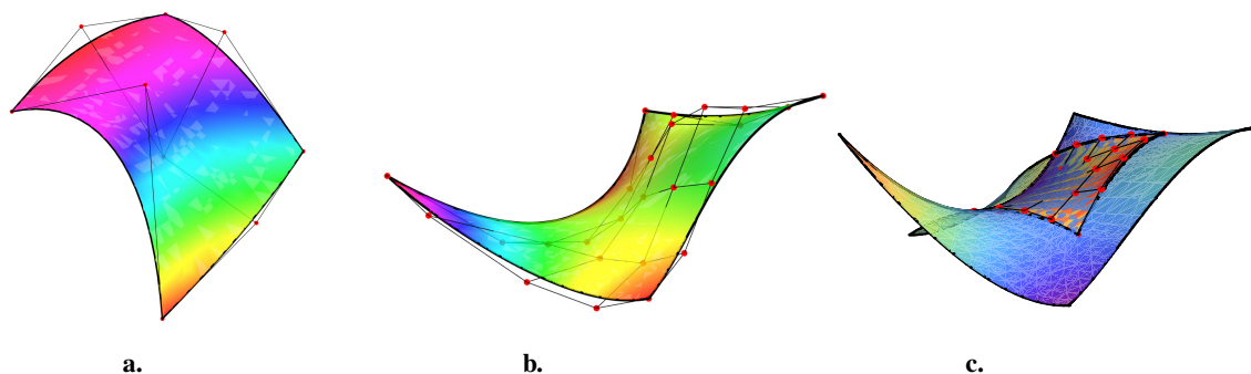
Figure 5: The irreducible TPB surfaces S_1 of degree (2, 2) and S_2 of degree (4, 4) and their coincident part S from Example 4. The corresponding control points are shown in Table 3. a. Surface S_1 ; b. Surface S_2 ; c. Surfaces S_1, S_2 , and S which is shown with its control polygon.
