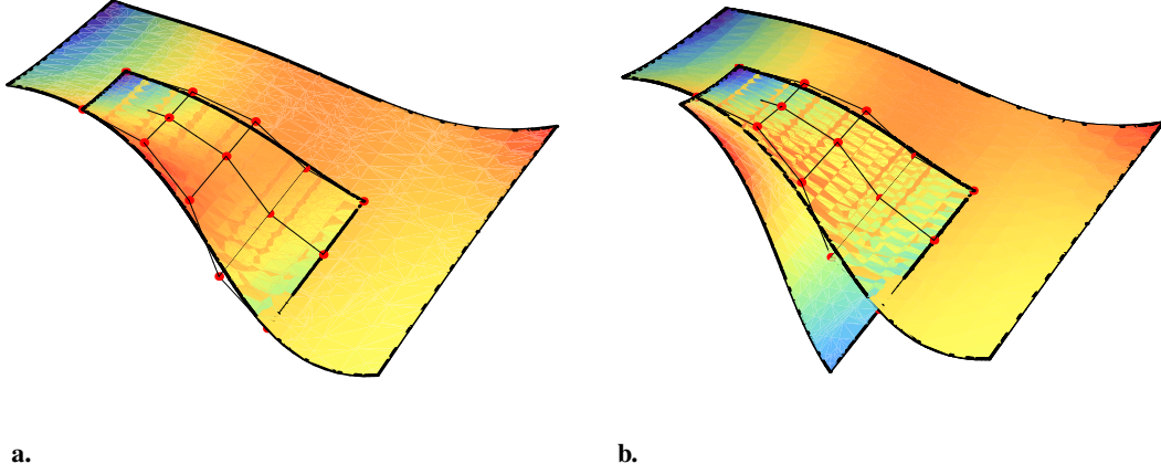
Figure 3: Testing for coincidence the surfaces shown in Fig. 2. a. Example 1: The coincident part of S_1 and S_2 is S_2 ; b. Example 2: The coincident part of S_1 and S_3 is S_2 .
