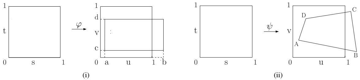
Figure 1: (i) The domain \{(u, v) : a \leq u \leq b, c \leq v \leq d\} is an image of the domain \{(s, t) : 0 \leq s \leq 1, 0 \leq t \leq 1\} under the affine transformation u = u(s) = (1-s)a + sb, v = v(t) = (1-t)c + td . (ii) The convex quadrilateral ABCD is an image of the domain \{(s, t) : 0 \leq s \leq 1, 0 \leq t \leq 1\} under a bilinear transformation.
