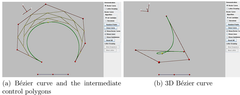
Figure 3: Bézier curves
