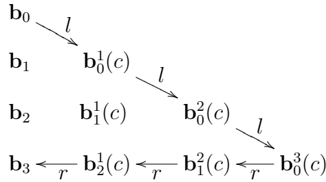
Figure 2: The control points of the left ( l ) and the right ( r ) cubic Bézier curves obtained after subdivision. The arrows indicate the ordering of the corresponding control points.
